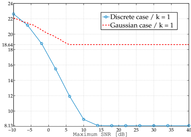
Fig. 2. Scenario a ; Plot of Expected payoff vs SNR for both the cases. One sees that the discrete strategy quickly beats the all-gaussian strategy, and achieves a much lower optimal cost
